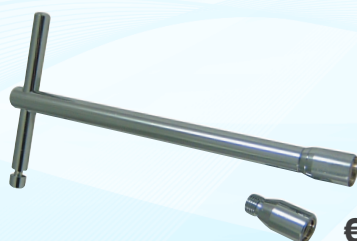
Hose protector installation tool. for 3/8 and 7/16 hoses. #SA05
