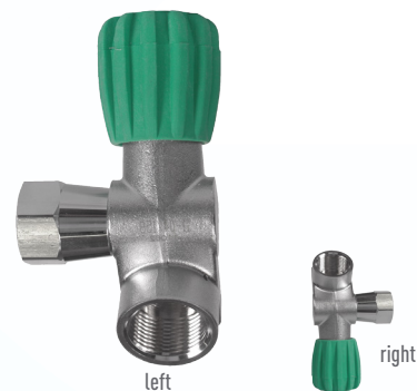
Second outlet M26 232 BAR M25x2 #N10098S left #N10099D right
