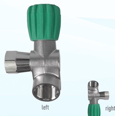
Second outlet M26 300 BAR M25x2 #N10098SD3 left #N10099DD3 right
